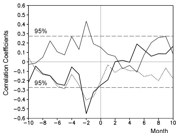
Fig. 9. Lag-correlation between autumn precipitation over South China and monthly SST anomalies in the western Pacific (thick solid curve), the North Pacific Ocean (dotted curve) and the South Indian Ocean (thin solid curve). The negative (positive) numbers on the x -axis represent the length of time the monthly SST anomalies lead (lag behind) autumn precipitation over South China. Dashed lines represent the 95% Student's t -test confidence level.
